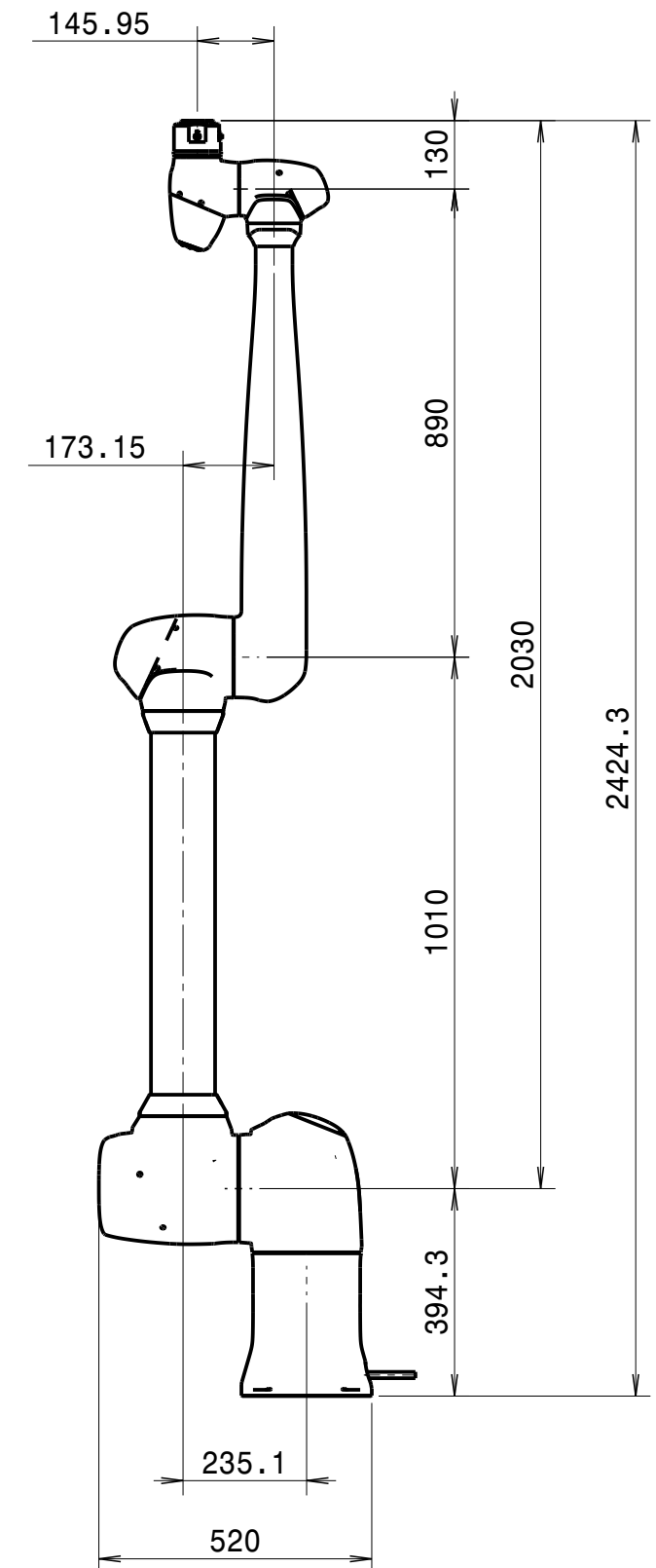
Side view (1:14)
