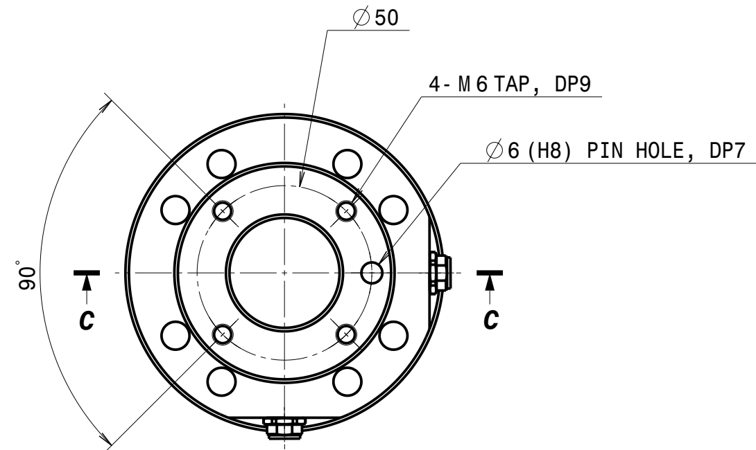
Tool flange (2:3)
