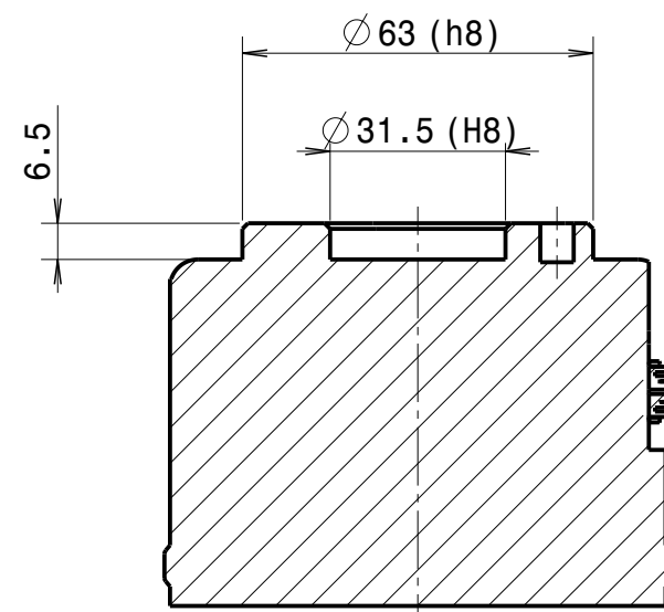
Section view C-C (2:3)
