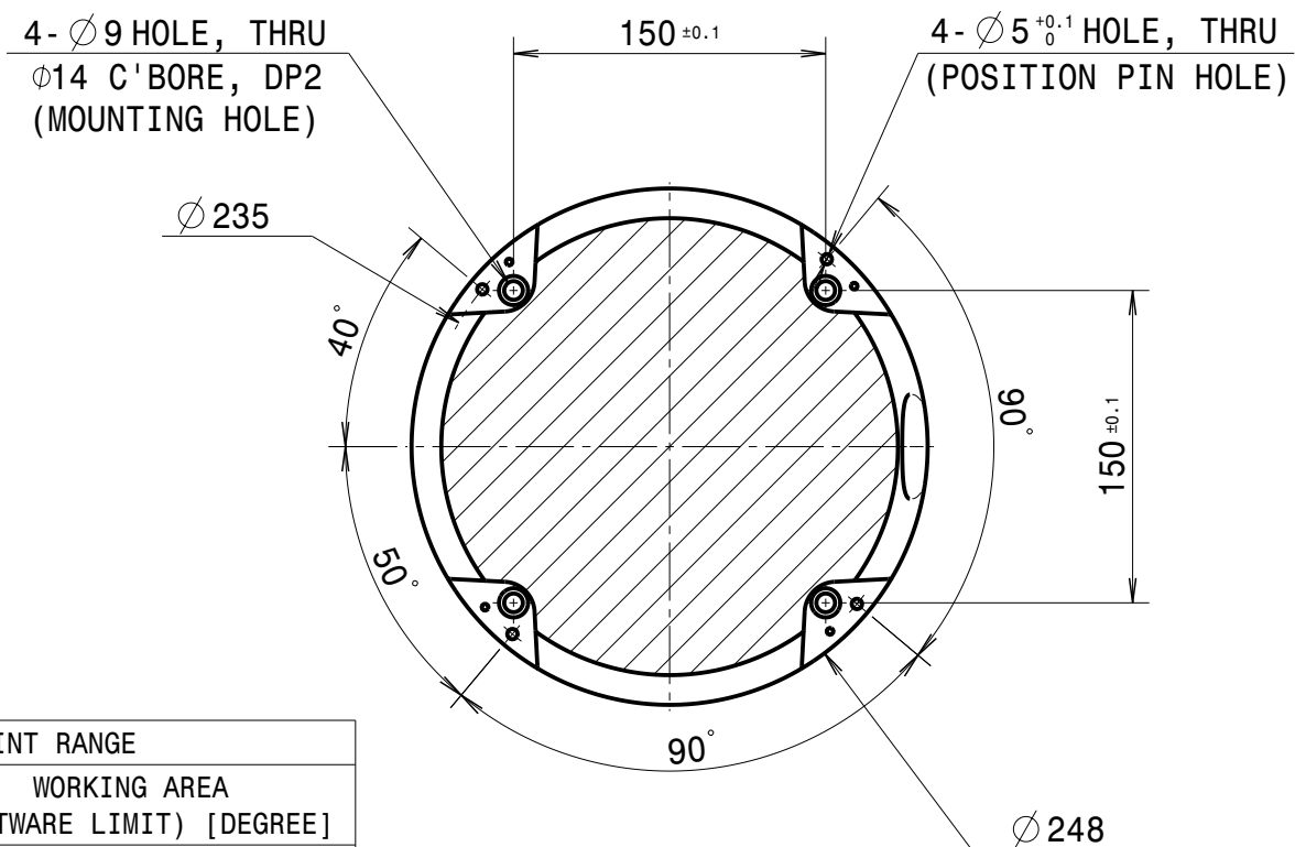
Section view A-A (1:4)
