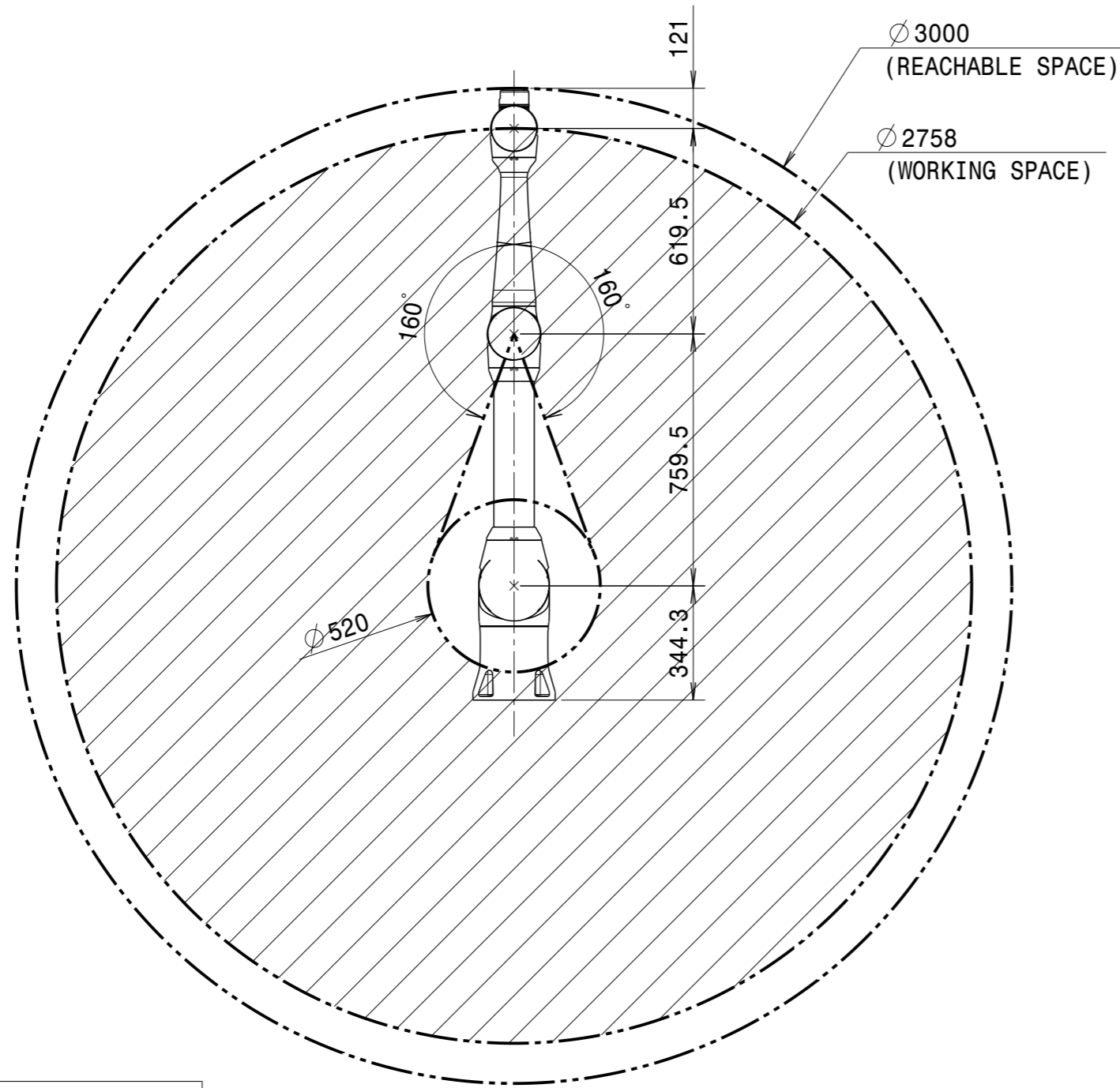
Front view (1:18)
