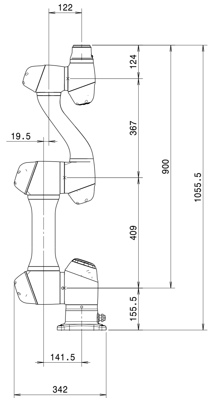
Side view (1:8)
