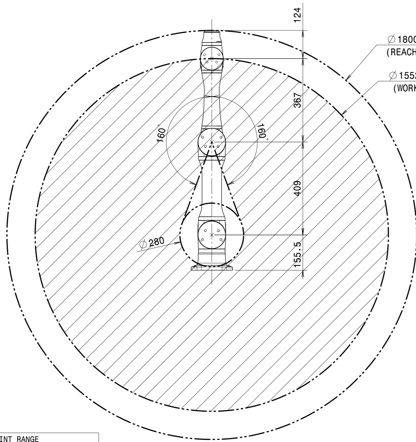
Front view (1:10)
